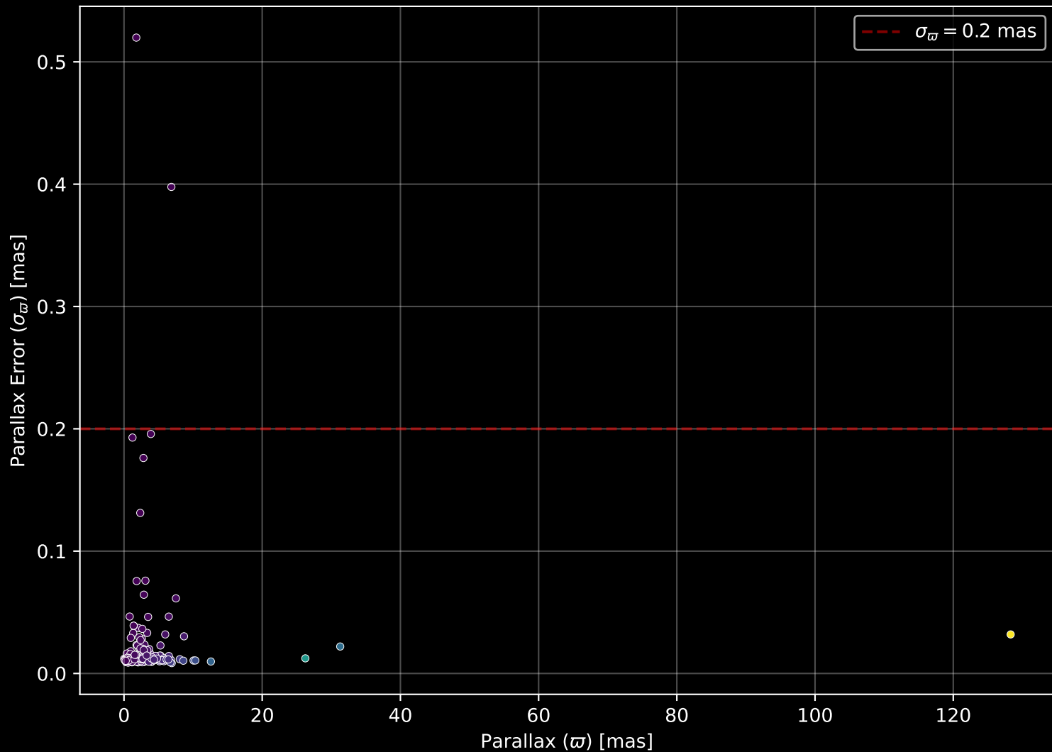
APOGEE DR17 Field: [CVZ_FILL01_btx] Parallax Quality (n= 185)
