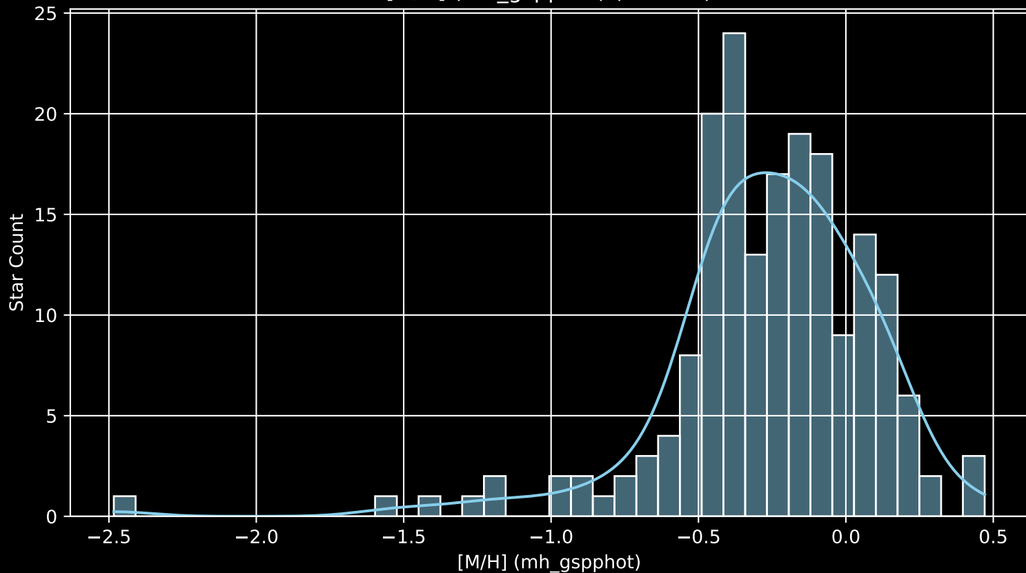
APOGEE DR17 Field: [CVZ_FILL01_btx [M/H] (mh_gspphot) (n= 185)
