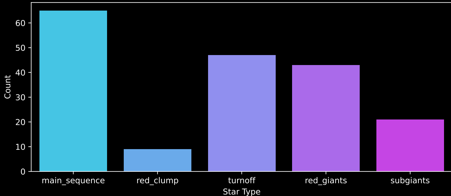
APOGEE DR17 Field: [CVZ_FILL01_btx] Count plot of Star Type
