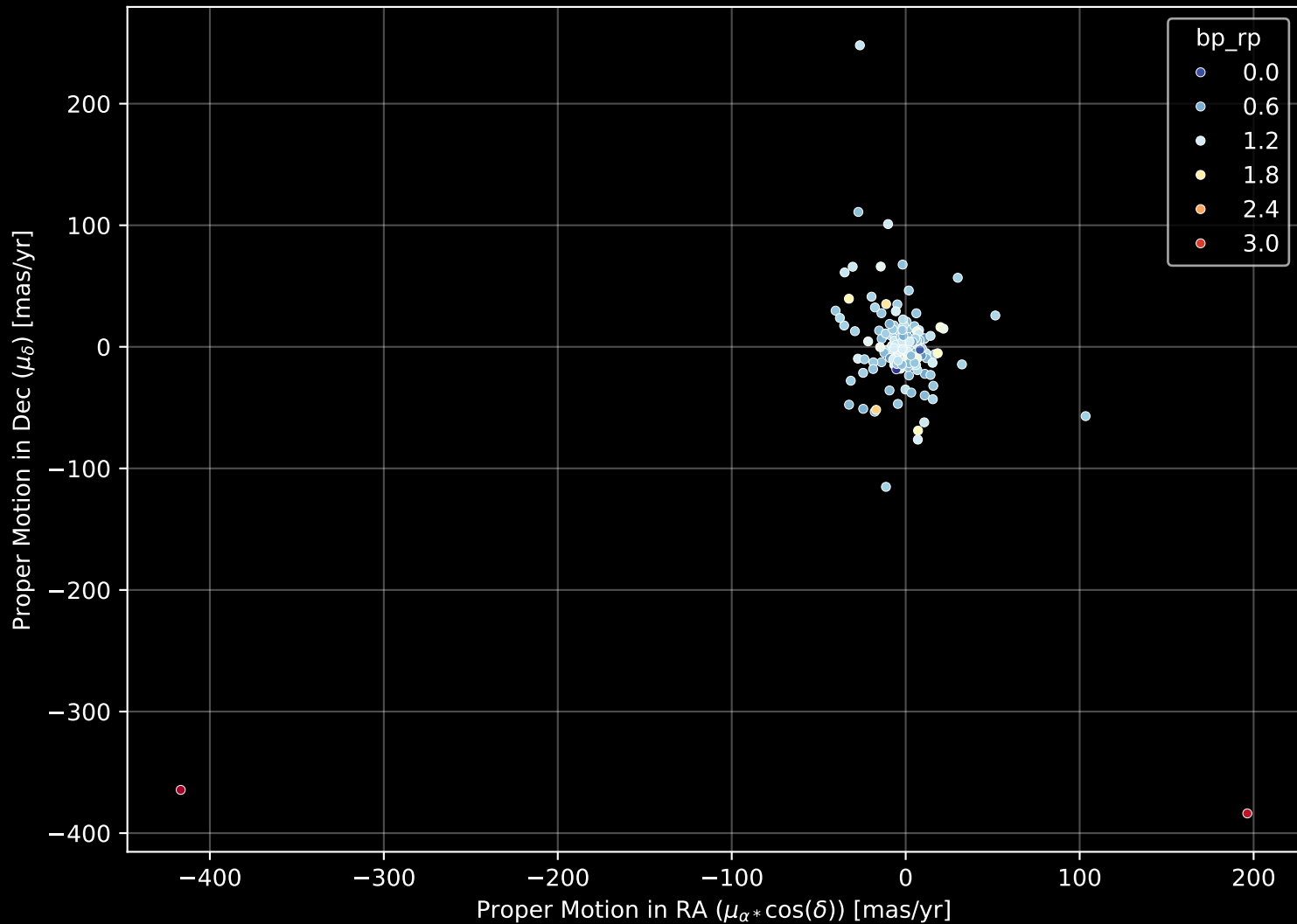
APOGEE DR17 Field: [CVZ_FILL01_btx] Proper Motion Diagram (n= 185)
