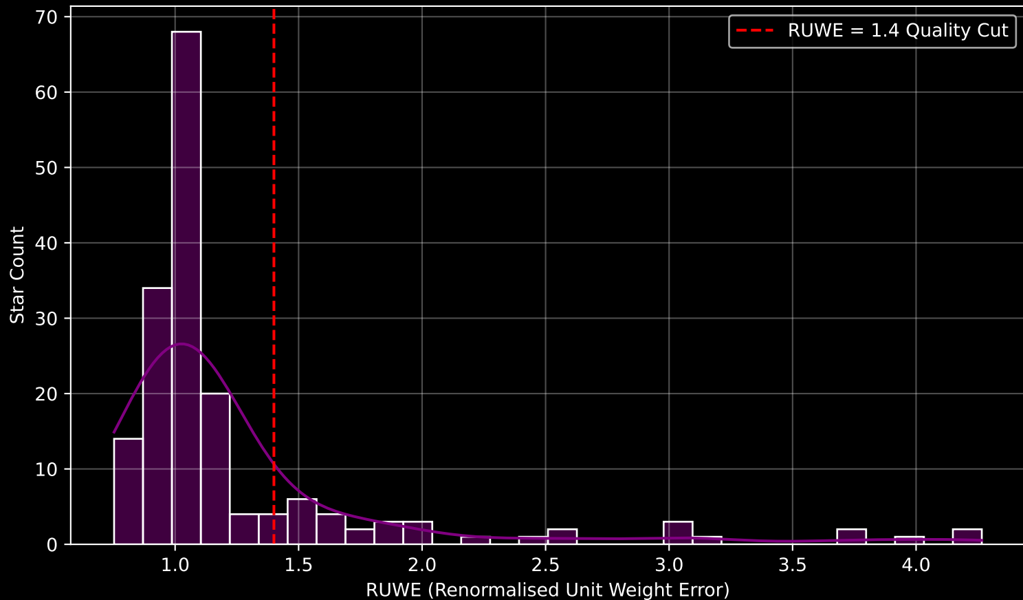
GAPOGEE DR17 Field [CVZ_FILL01_btx] RUWE Distribution (n= 175)
