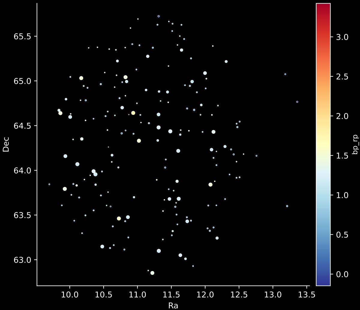
APOGEE DR17 Field: [CVZ_FILL01_btx] Stars: 185
